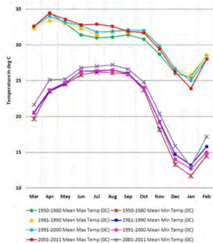
Figure 8: Monthly Mean Maximum and Minimum Air temperature profile for the year 1950-1980, 1981-1990, 1991-2000, and 2001-2011. Source: (Bangladesh Meteorological Department, Dhaka, 2012)
