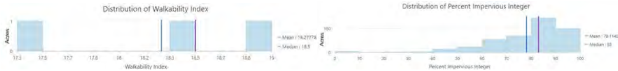
Figure 14: The histogram above describes the National Walkability Index rankings within the block groups included in the downtown Boulder, Colorado boundary. Figure 15: The distribution of percent impervious surface per acre of downtown West Palm Beach, Florida.
