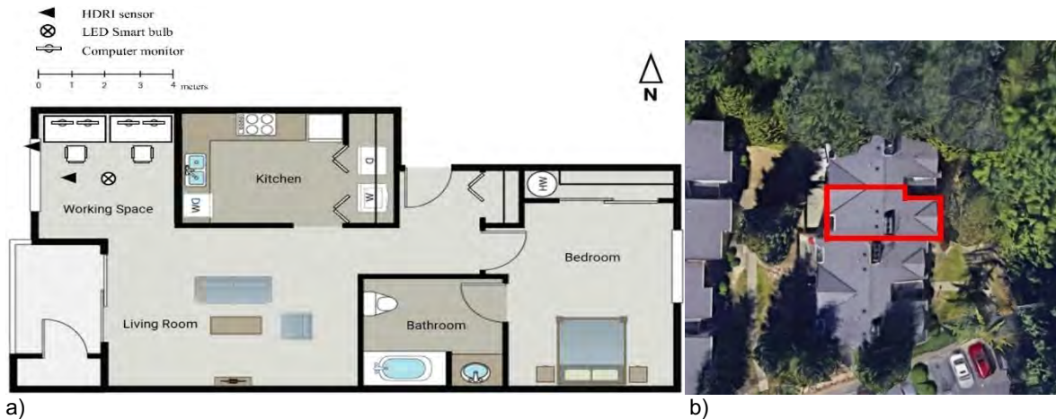
Figure 1: Example of home-office layout. a) plan shows where the subjects were seated, positions of computer monitors, LED smart bulb, and locations and view orientations of HDRI sensors, b) surrounding urban context.
