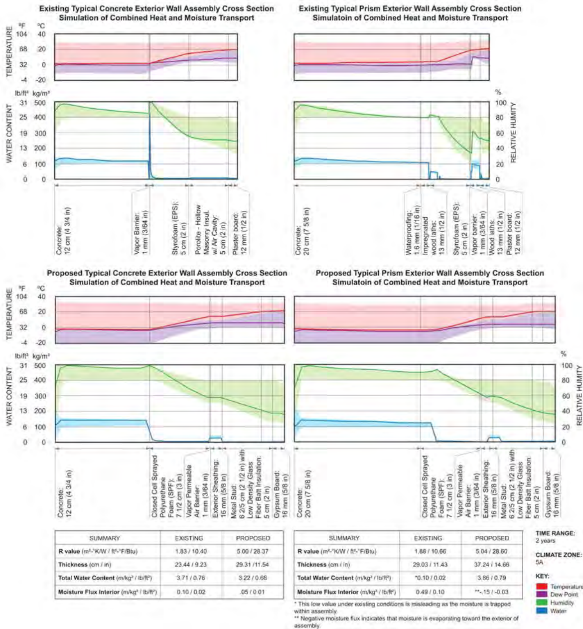
Figure 9: Thermal and moisture transfer analysis of two selected exterior wall assemblies at Spomen Dom .
