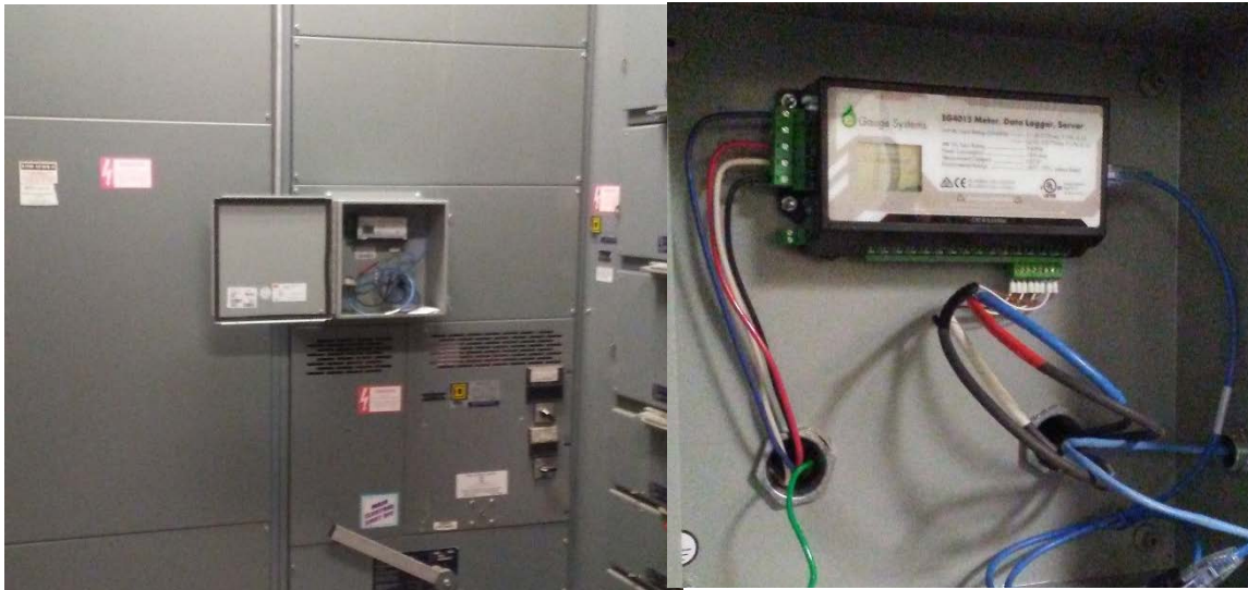
Figure 3: Installed eGauge data logger unit and associated wiring for Automated Energy Use Data Collection and Visualization for Game-based Education
