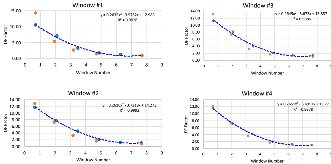
Figure 4: Evaluation of daylight factor at each window in both simulation by ALFA and physical model The calibration also exhibits in (Figure 5) with 0.988963 correlation and 1.0536 calibration factor.
