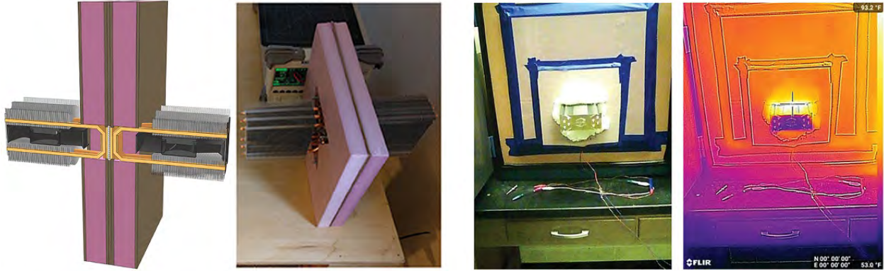
Figure 1: Experimental prototype and thermal imaging. Source: (Author 2018)
